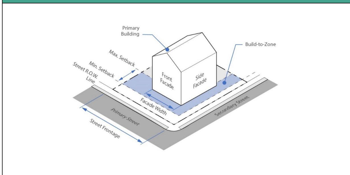
DIAGRAM 9.3.A.4 PRIMARY AND SECONDARY BUILD-TO-ZONE (BTZ)
